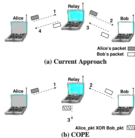
Figure 1—A simple example of how COPE increases the throughput. It allows Alice and Bob to exchange a pair of packets using 3 transmissions instead of 4 (numbers on arrows show the order of transmission).
